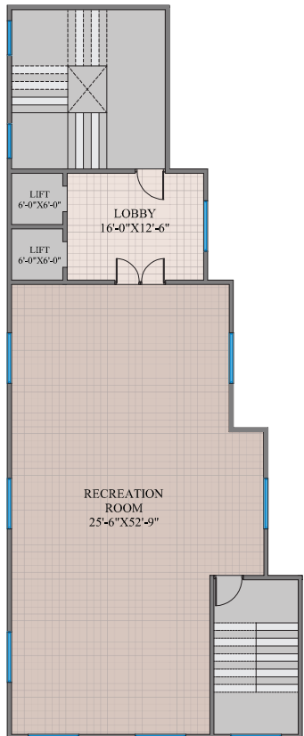
FIFTH FLOOR PLAN
