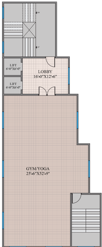
FOURTH FLOOR PLAN
